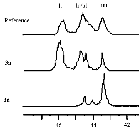
Figure 3. Comparative 13 C NMR spectrum of the copolymers in the region of the methylene carbon atom using the epimerized copolymer as reference
