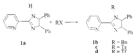
Figure 1. Synthesis of the pyridine-imidazoline ligands
