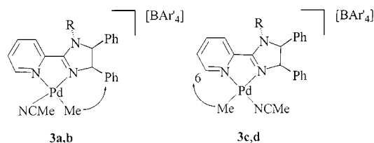
Figure 2. NOE difference experiments show the stereochemistry of the complexes
